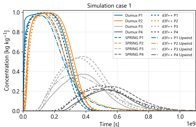
Figure A1. Landfill model concentration curves for simulation case 1 ( \alpha_l = 0.1 m and K_d = 0 m 3 kg -1 ) with full upwind in d 3 f++ at different observation points.
