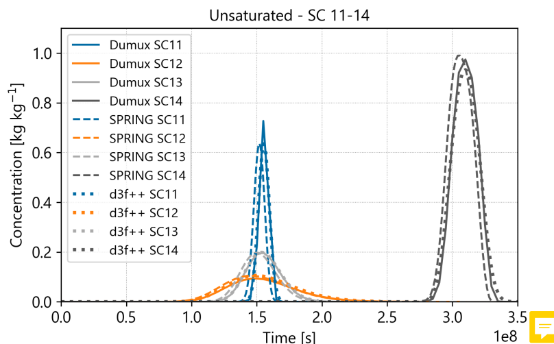
Figure 6. Concentration breakthrough curves for the simulation cases 11 to 14 (unsaturated cases) for the three different Codes DuMu x (solid line), d 3 f++ (dotted line) and SPRING (dashed line). Blue curve: advective transport; orange curve: advection and dispersion; grey curve: advection and diffusion; black curve: advection and sorption.
