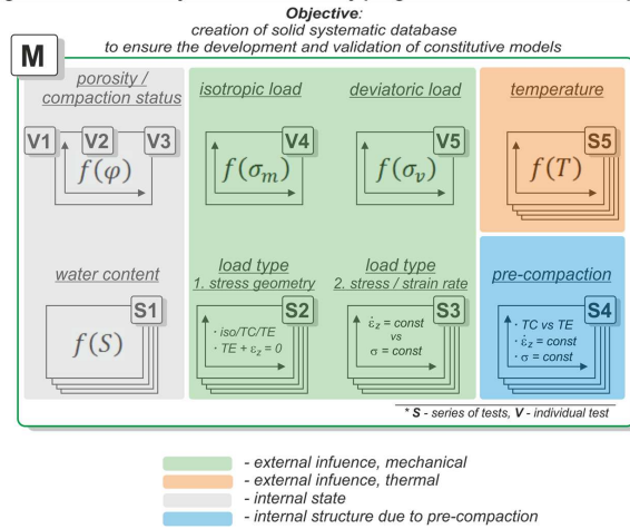
135 Figure 3: Systematic laboratory program as a basis for building the experimental database in the crushed salt projects.
