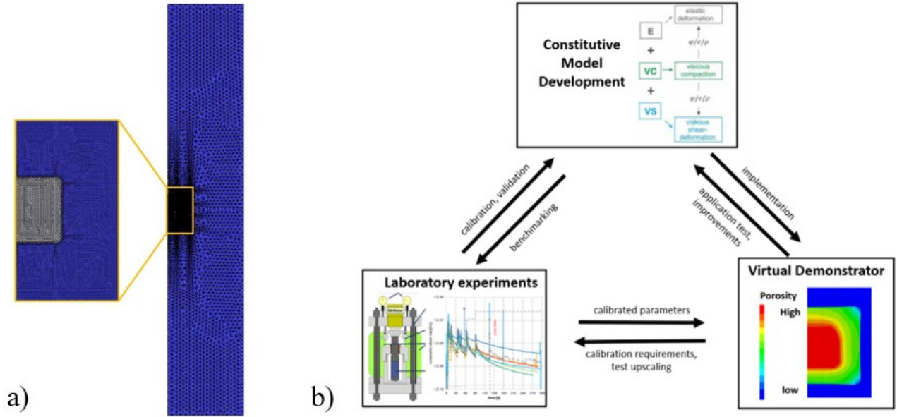
160 Figure 4: Virtual demonstrator. a) Numerical model of a generic backfilled drift in rock salt. b) Conceptual illustration of the role of the virtual demonstrator.
