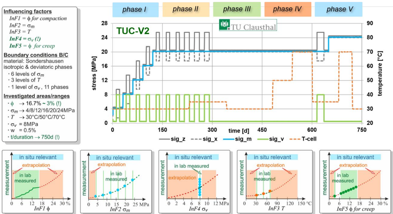
195 Figure 5: Thermomechanical loading program TUC-V2 applied in the long-term laboratory investigation of crushed salt compaction (Friedenberg et al., 2024)
